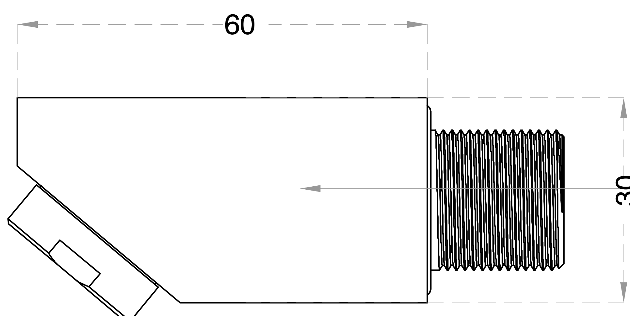
SIDE ELEVATION
