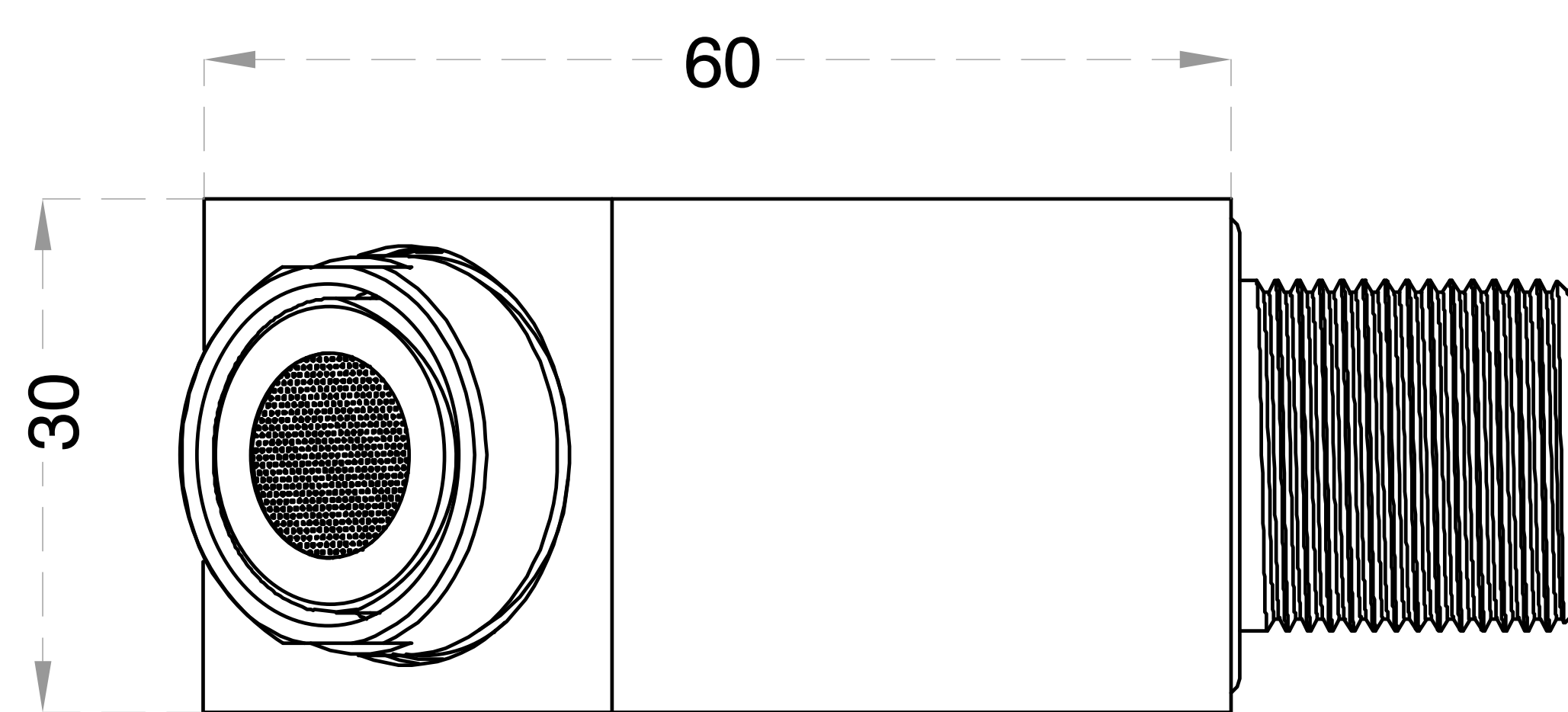
PLAN
